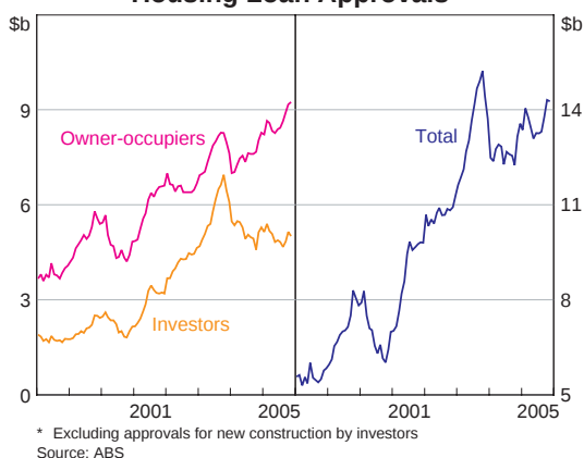
Graph 31 Housing Loan Approvals*
