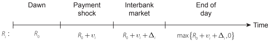
Figure 7: Time Line
